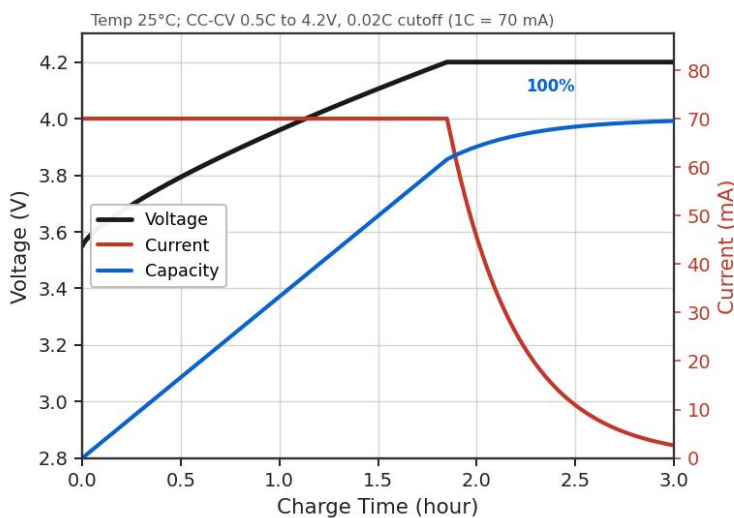
Charging Characteristic
