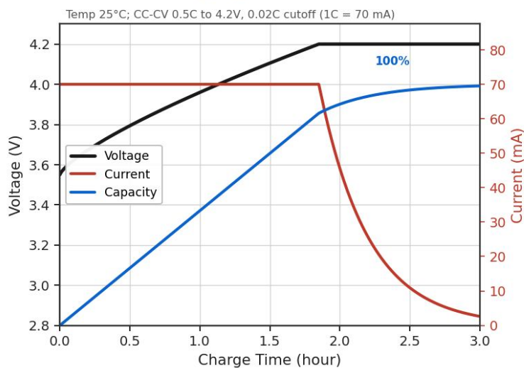
Charging Characteristic
