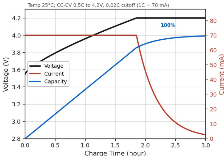
Charging Characteristic
