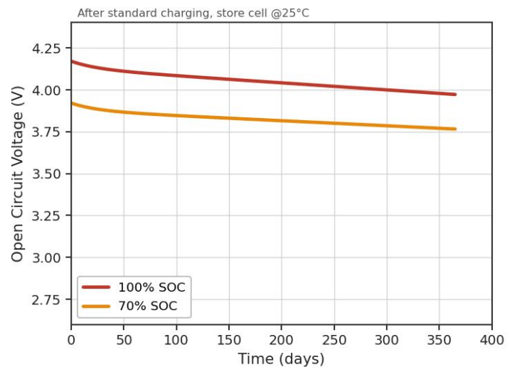
Self-Discharge at Different SOC
