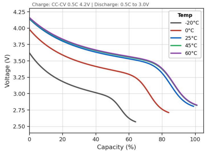
Discharge Curve at Different Temperatures
