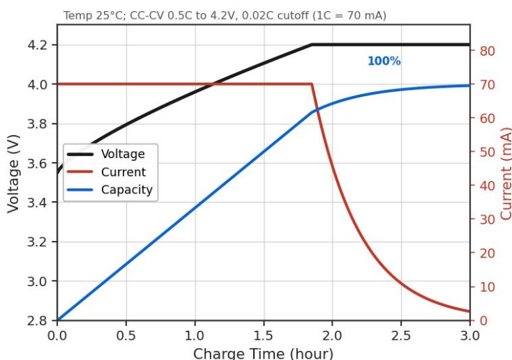
Charging Characteristic
