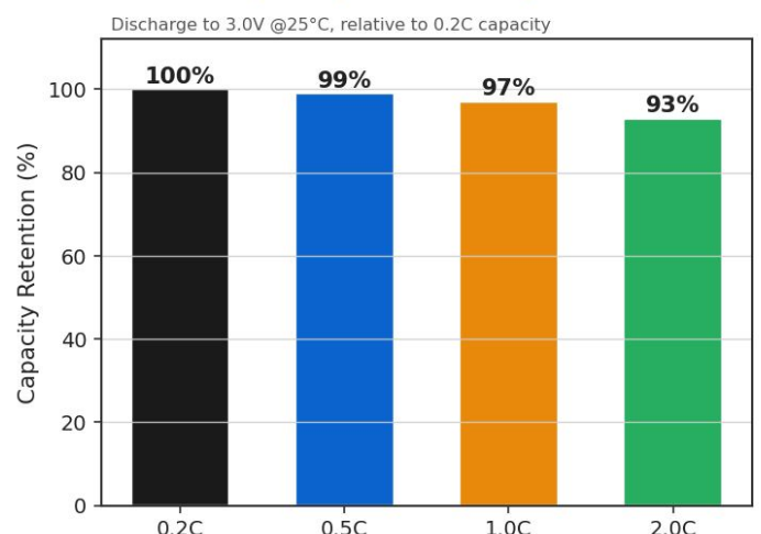
Capacity vs Discharge Rate
