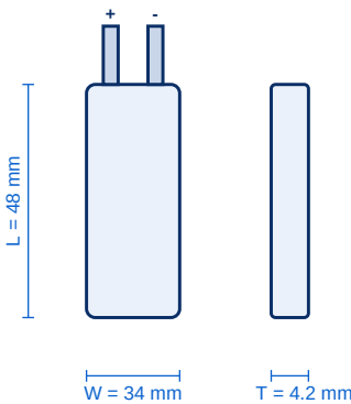
Cell Dimension Sketch
