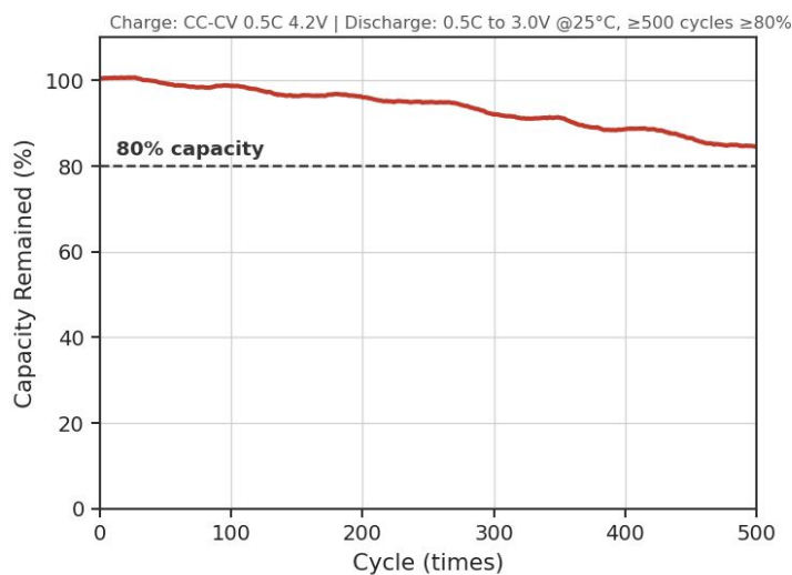
Cycle Life Curve
