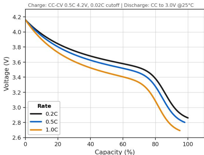
Discharge Curve at Different Rates
