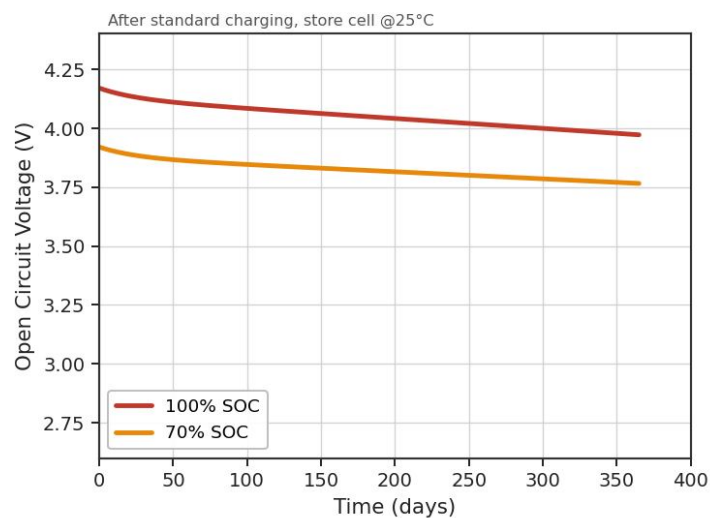
Self-Discharge at Different SOC
