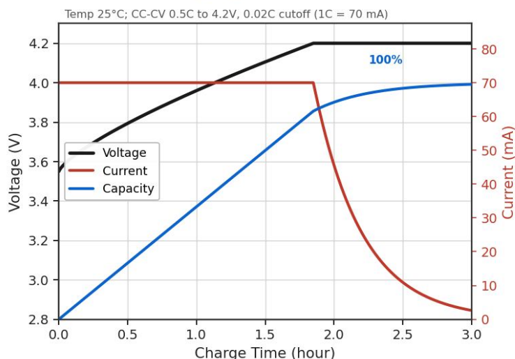
Charging Characteristic
