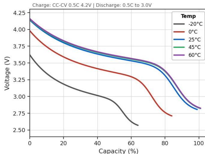
Discharge Curve at Different Temperatures
