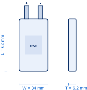
Cell Dimension Sketch
