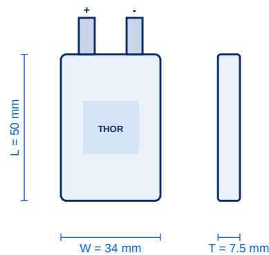
Cell Dimension Sketch
