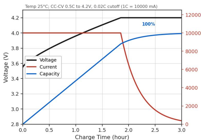
Charging Characteristic
