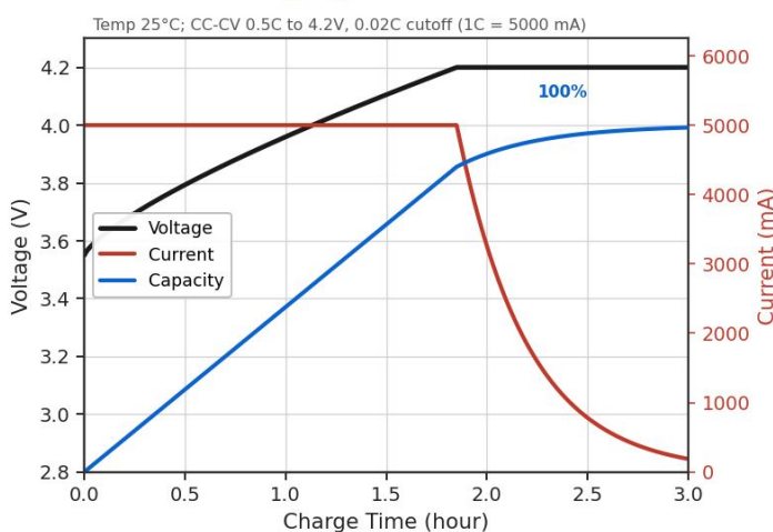
Charging Characteristic
