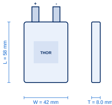
Cell Dimension Sketch
