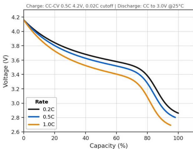
Discharge Curve at Different Rates
