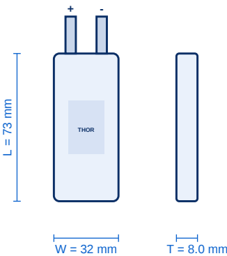
Cell Dimension Sketch
