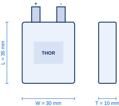
Cell Dimension Sketch
