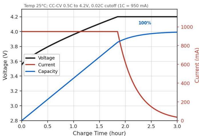
Charging Characteristic
