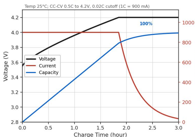
Charging Characteristic
