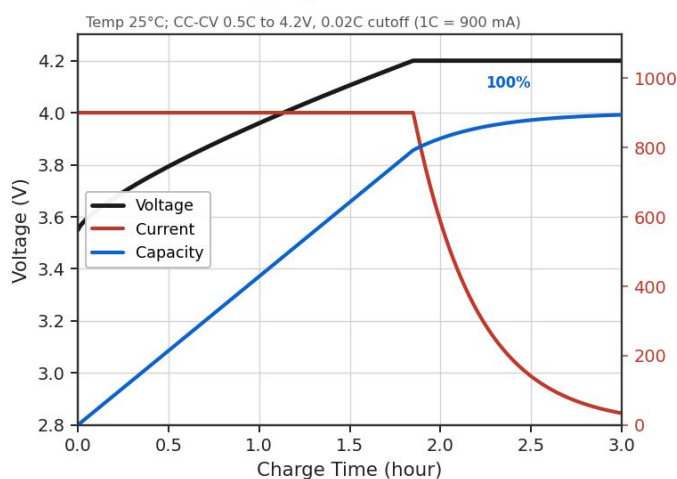
Charging Characteristic
