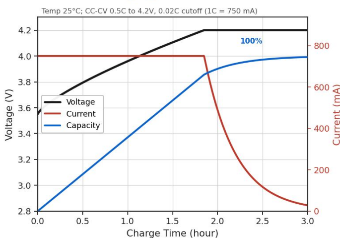
Charging Characteristic
