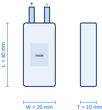
Cell Dimension Sketch
