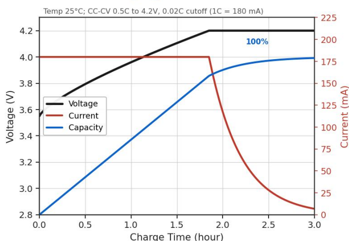
Charging Characteristic
