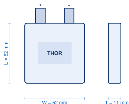
Cell Dimension Sketch
