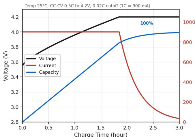
Charging Characteristic
